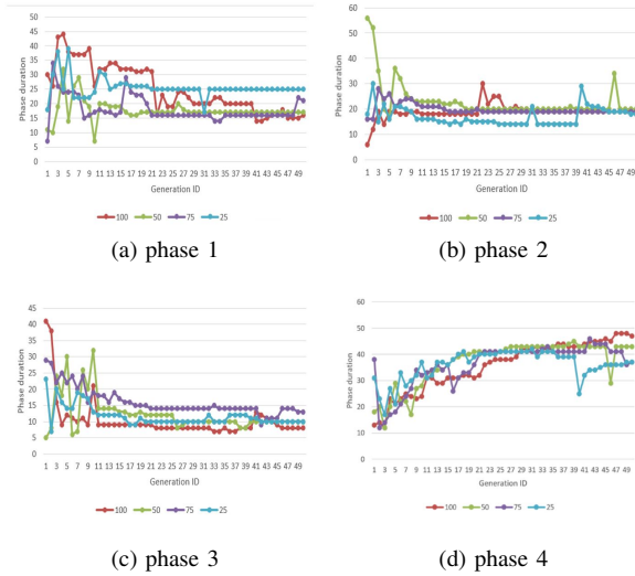
Figure 1. Phase duration convergence in intersection 2
