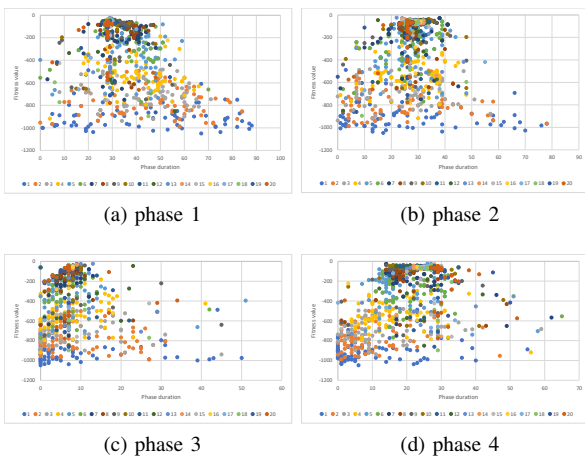
Figure 8. Phase duration convergence in intersection 4
